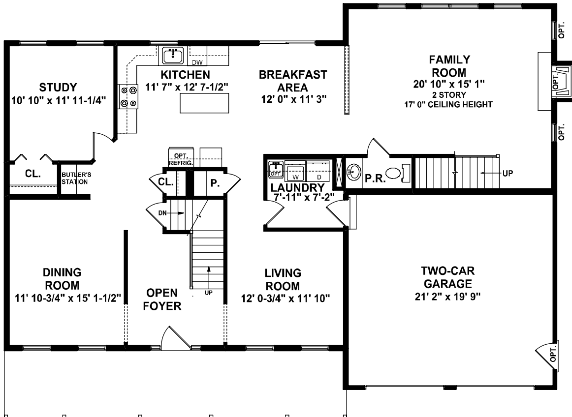
FIRST FLOOR
