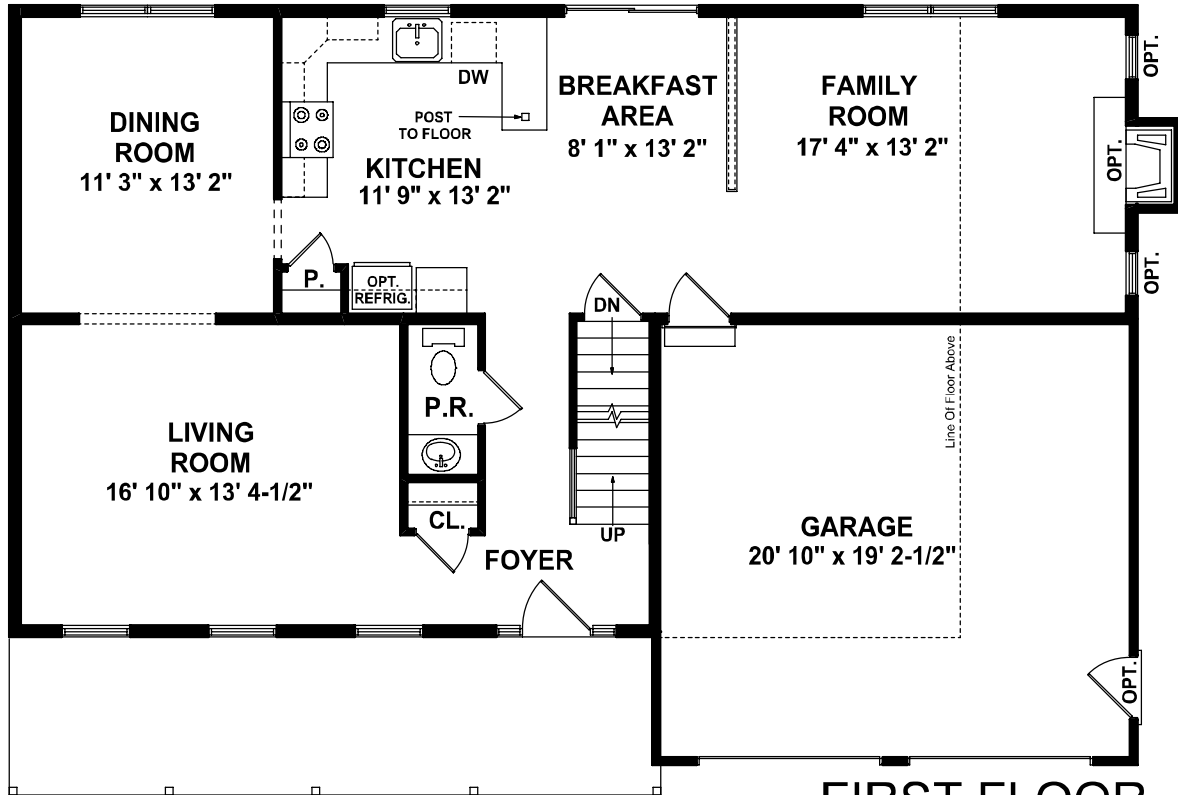
FIRST FLOOR
